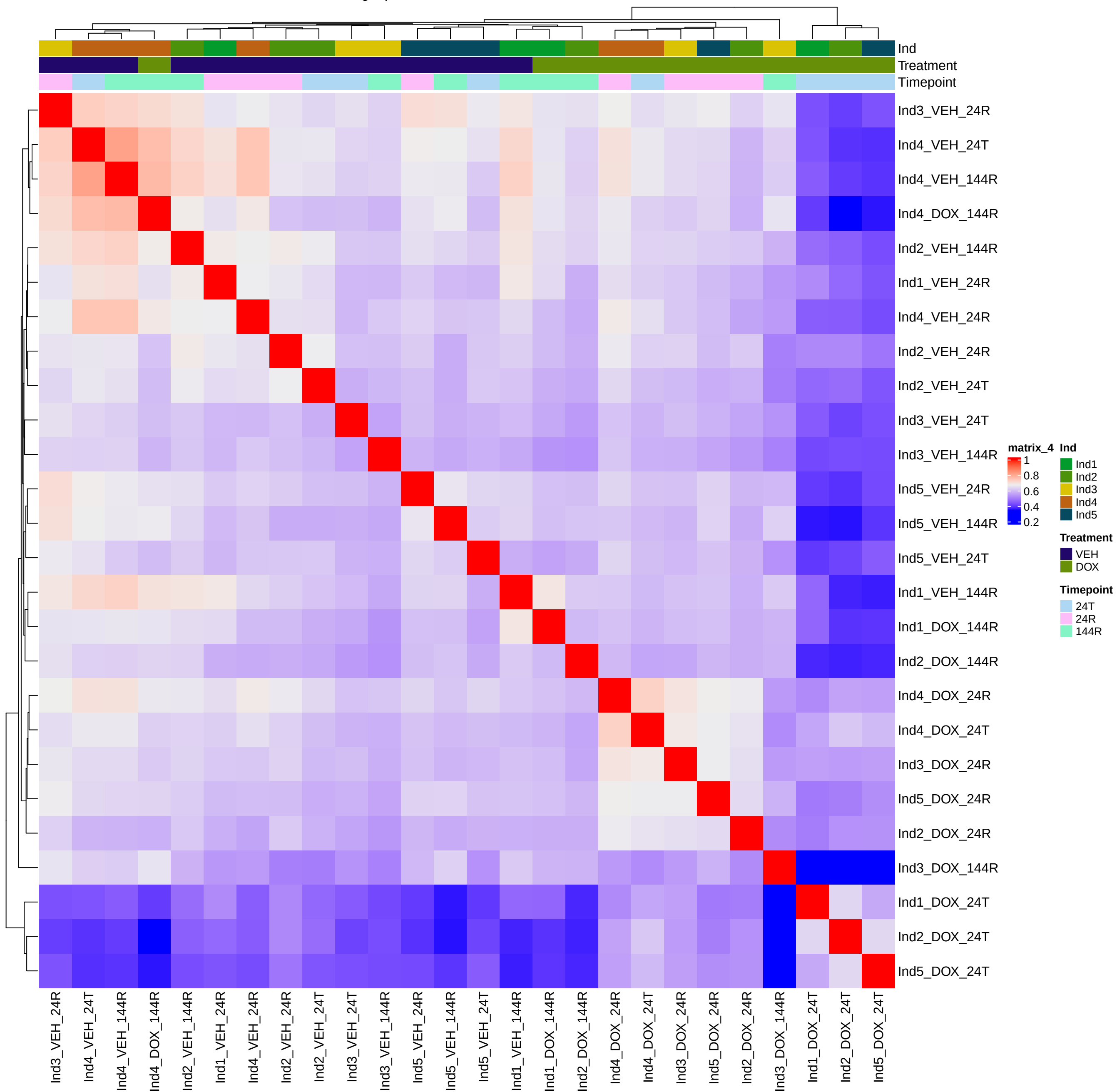
Filtered log2cpm H3K9me3 with removal of 3 outliers
